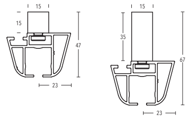
Ceiling bracket 15 mm + 35 mm Art. no. 11473-15 + 11473-35
