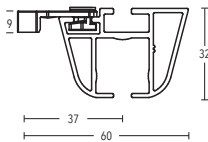
Clamping ceiling bracket 3 mm Art. no. 11590-10-00
