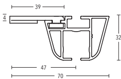
Ceiling bracket 3 mm Art. no. 11592
