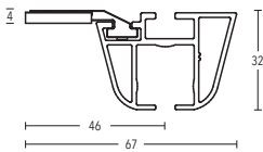
Ceiling bracket 3 mm Art. no. 11597
