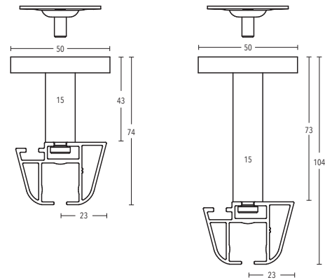
Ceiling bracket 43 mm + 73 mm Art. no. 11473-50 + 11473-80
