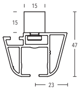
Ceiling bracket 15 mm Art. no. 11473-100
