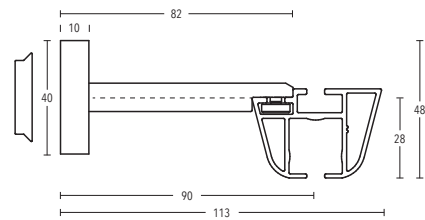
Wall bracket Art. no. 11260-90
