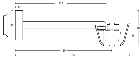
Wall bracket Art. no. 11260-130
