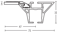
Ceiling bracket 3 mm Art. no. 11597-00
