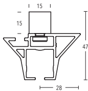
Ceiling bracket 15 mm Art. no. 11473-100
