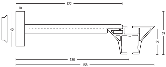
Wall bracket Art. no. 11260-130
