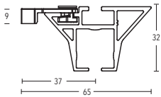
Clamping ceiling bracket 3 mm Art. no. 11590-10-00
