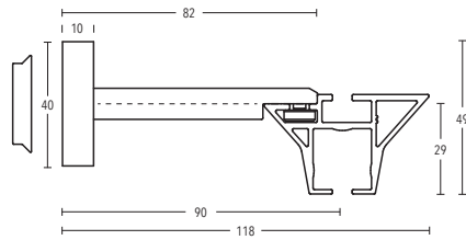
Wall bracket Art. no. 11260-130
