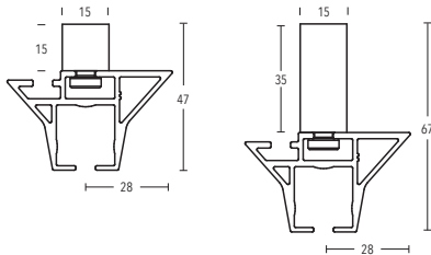
Ceiling bracket 15 mm + 35 mm Art. no. 11473-15 + 11473-35
