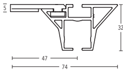
Ceiling bracket 3 mm Art. no. 11592-00
