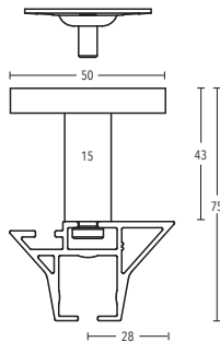
Ceiling bracket 43 mm + 73 mm Art. no. 11473-50 + 11473-80
