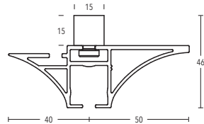
Ceiling bracket 15 mm + 35 mm Art. no. 11473-15 + 11473-35
