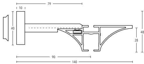
Wall bracket Art. no. 11220-90
