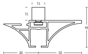
Ceiling bracket 15 mm Art. no. 11473-100
