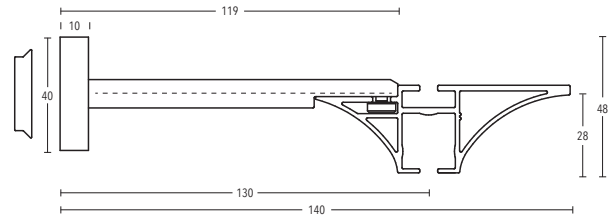
Wall bracket Art. no. 11220-130
